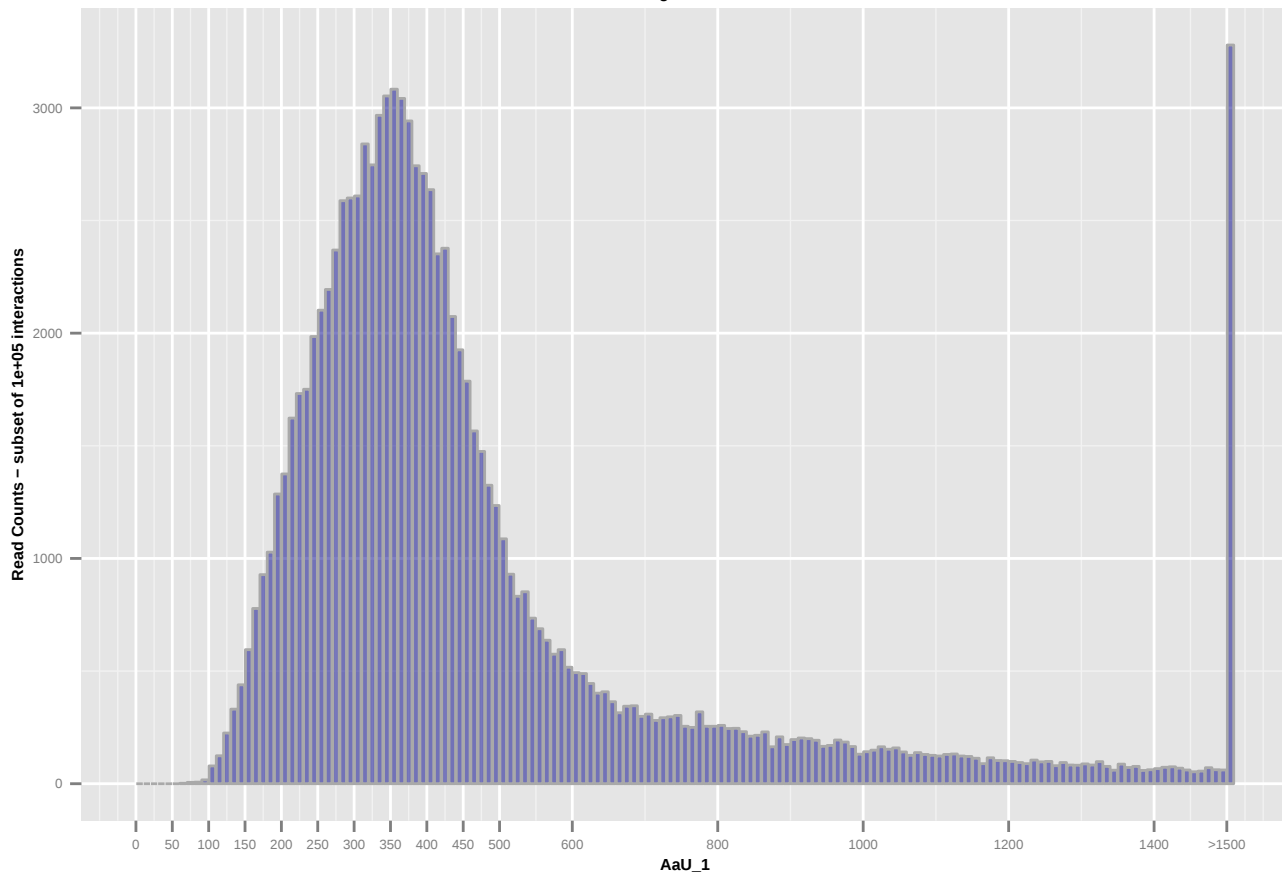
Valid Pairs - Fragment size distribution
