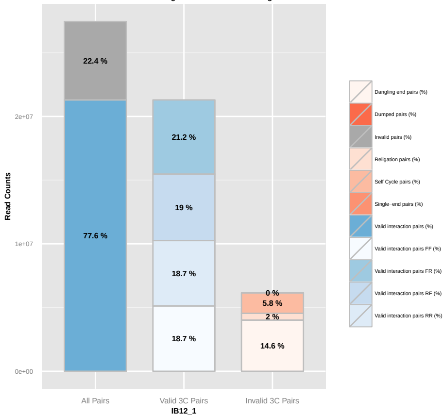
Statistics of Read Pairs Alignment on Restriction Fragments
