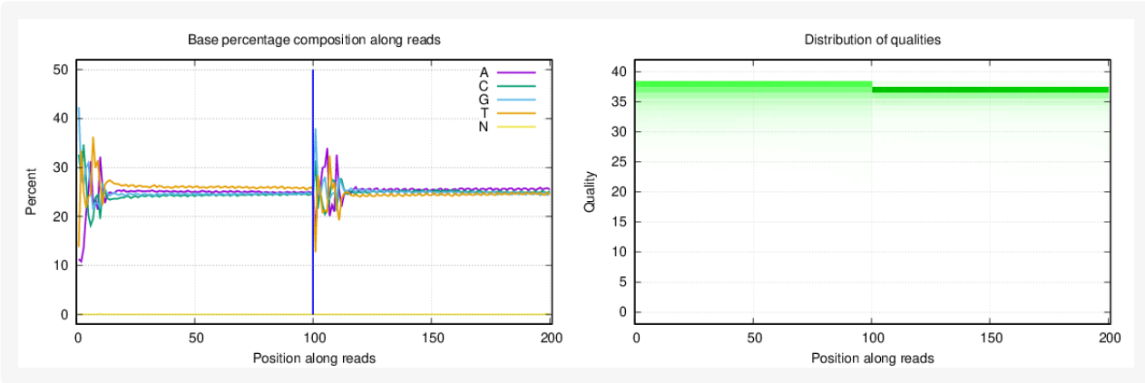
Figure 1-4 Distribution of base percentage and qualities of sample N9.
