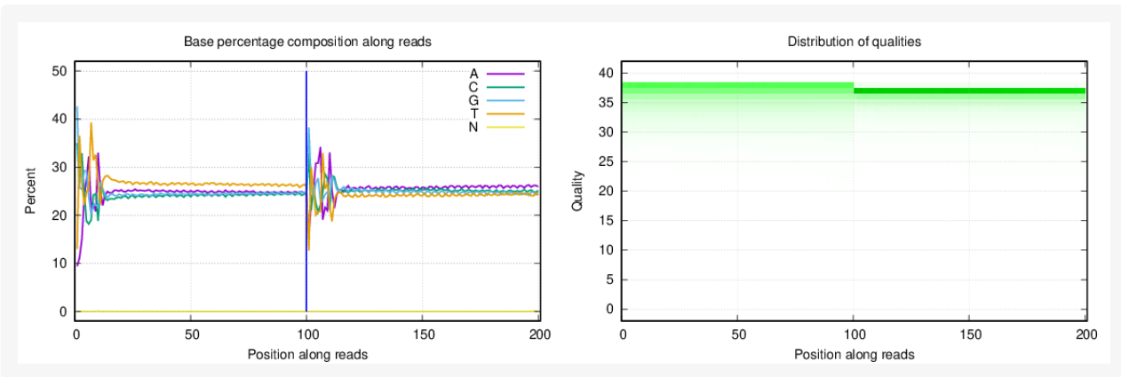
Figure 1-27 Distribution of base percentage and qualities of sample 7G4.
