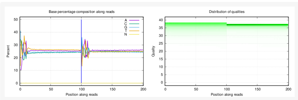
Figure 1-9 Distribution of base percentage and qualities of sample N4.
