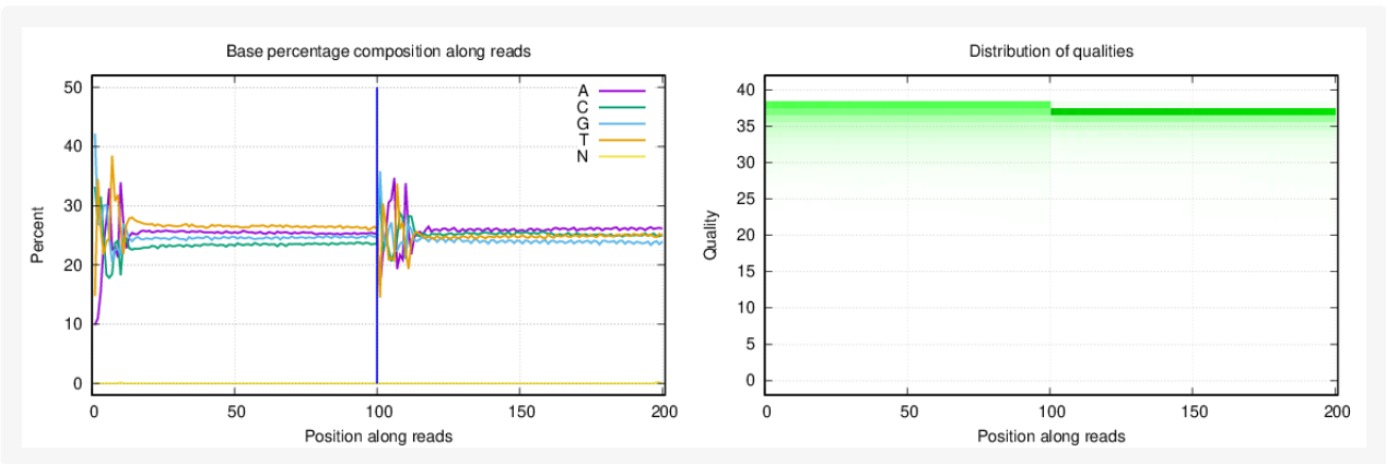
Figure 1-24 Distribution of base percentage and qualities of sample E1.
