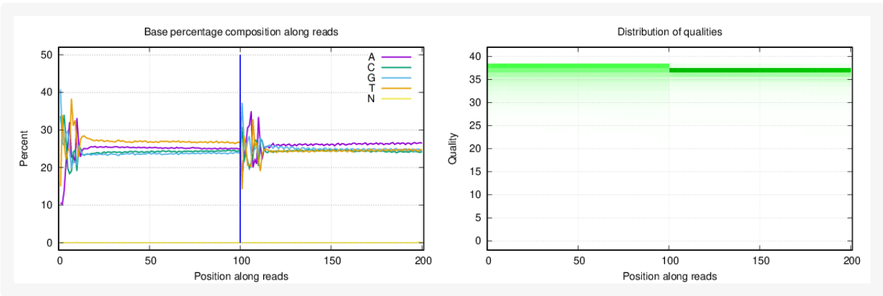
Figure 1-22 Distribution of base percentage and qualities of sample E3.
