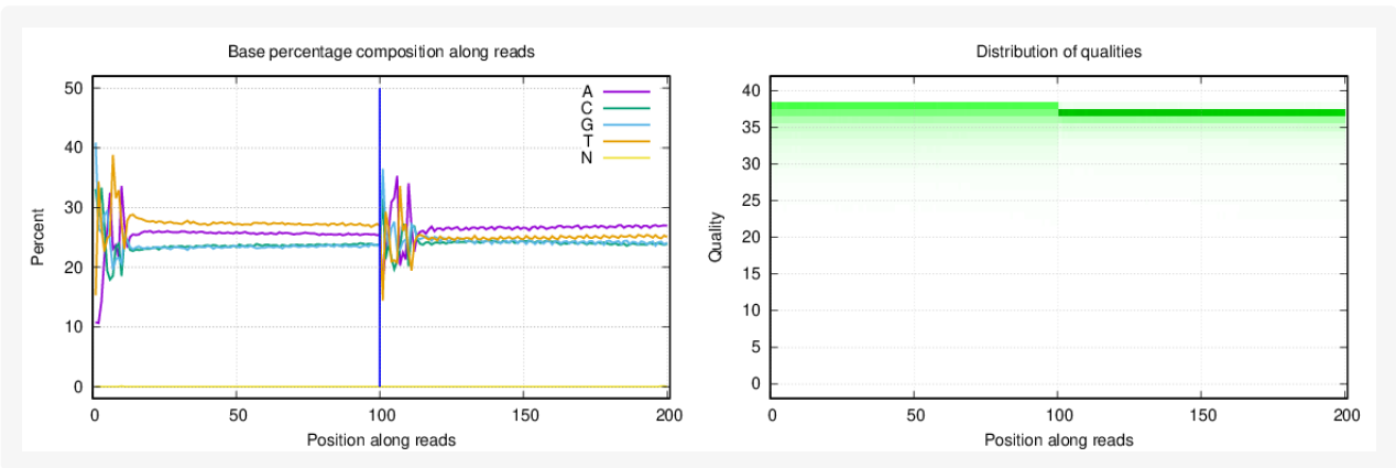
Figure 1-21 Distribution of base percentage and qualities of sample E4.
