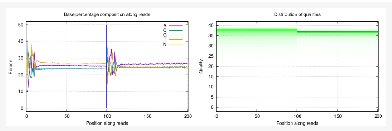
Figure 1-18 Distribution of base percentage and qualities of sample E7.
