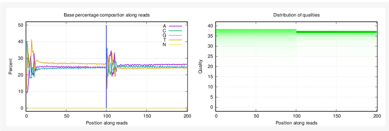
Figure 1-26 Distribution of base percentage and qualities of sample 7VPR.
