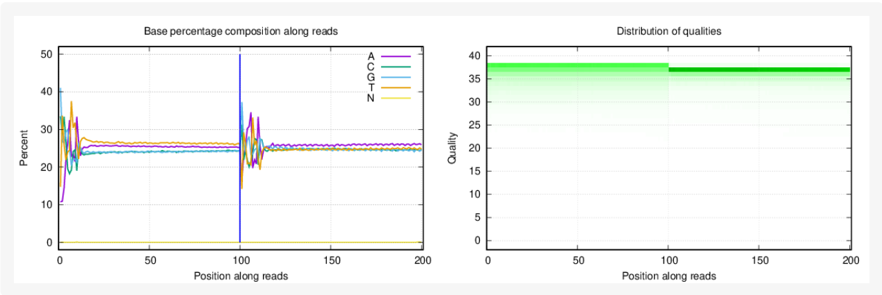
Figure 1-15 Distribution of base percentage and qualities of sample E10.
