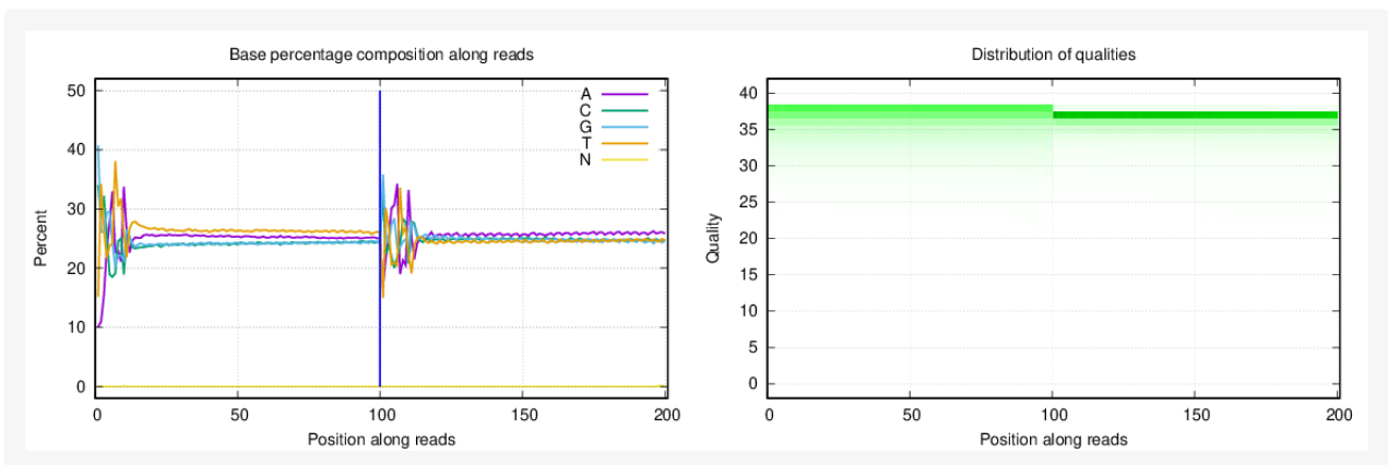
Figure 1-33 Distribution of base percentage and qualities of sample 14TR11.
