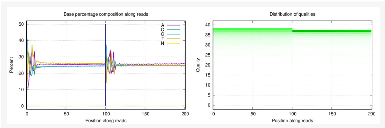
Figure 1-3 Distribution of base percentage and qualities of sample N10.
