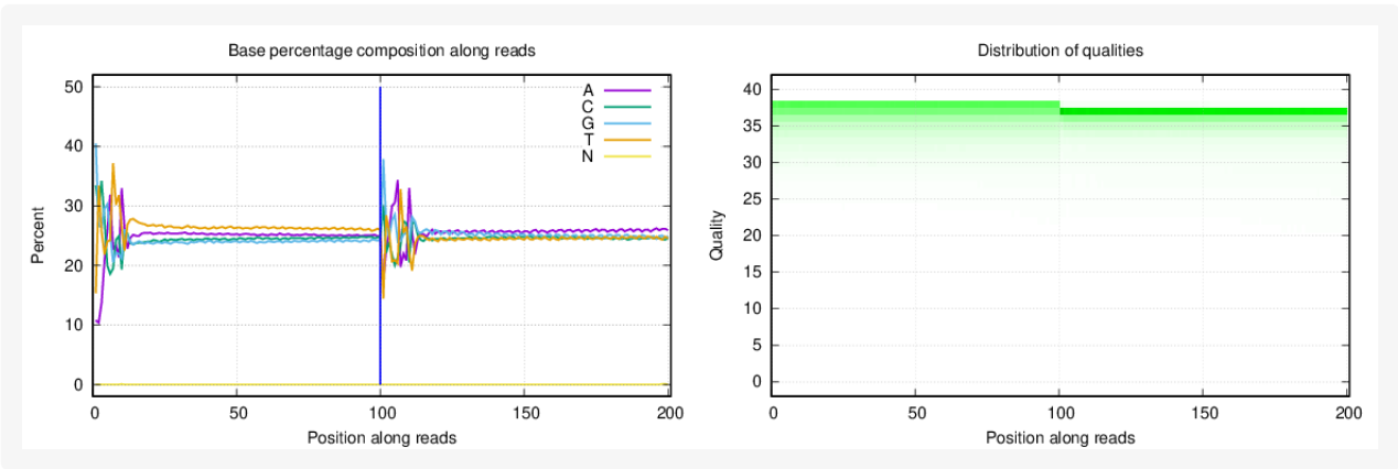
Figure 1-28 Distribution of base percentage and qualities of sample 15DR8.
