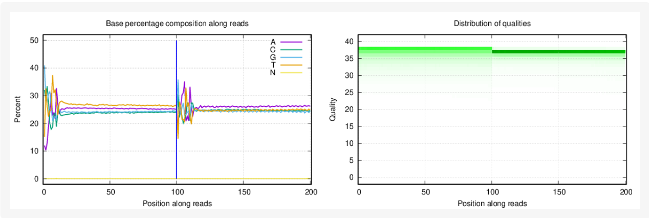
Figure 1-16 Distribution of base percentage and qualities of sample E9.
