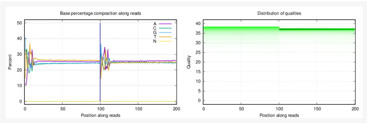
Figure 1-7 Distribution of base percentage and qualities of sample N6.
