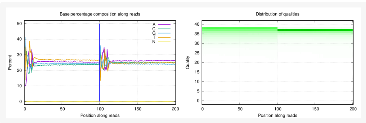
Figure 1-23 Distribution of base percentage and qualities of sample E2.
