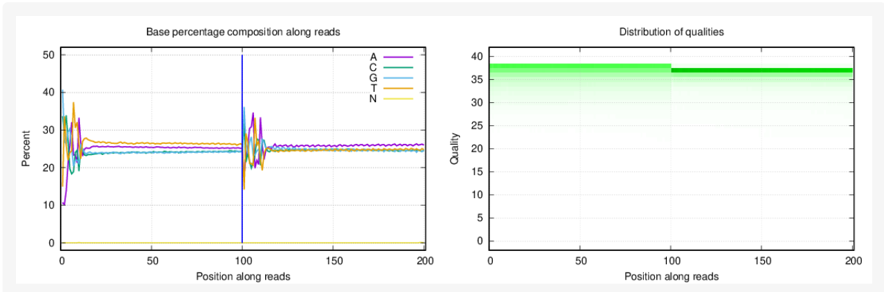
Figure 1-2 Distribution of base percentage and qualities of sample N11.
