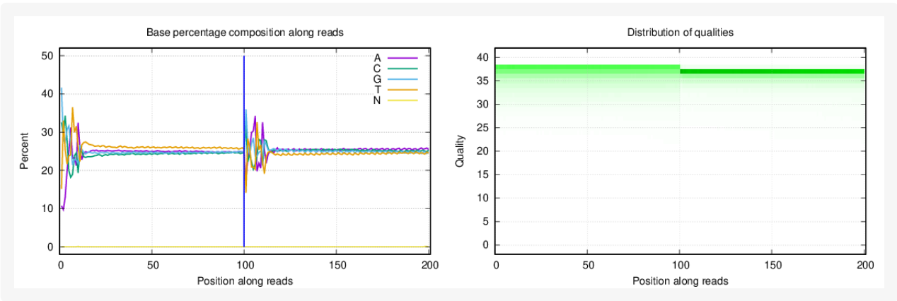
Figure 1-10 Distribution of base percentage and qualities of sample N3.
