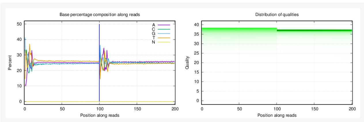
Figure 1-8 Distribution of base percentage and qualities of sample N5.
