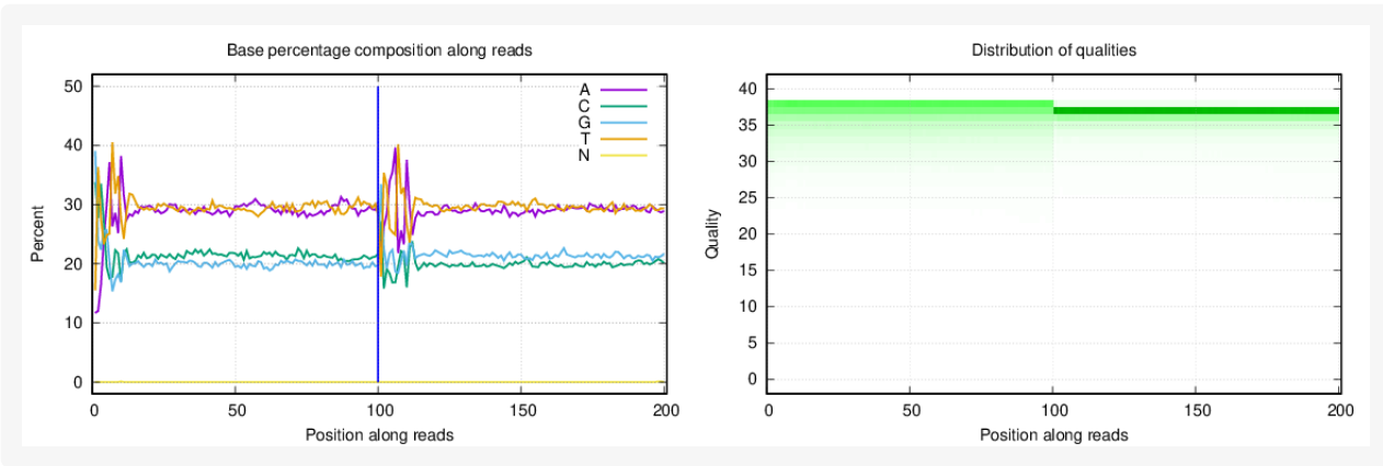
Figure 1-25 Distribution of base percentage and qualities of sample SN.
