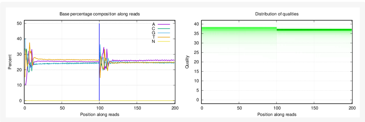
Figure 1-29 Distribution of base percentage and qualities of sample 14DR7.
