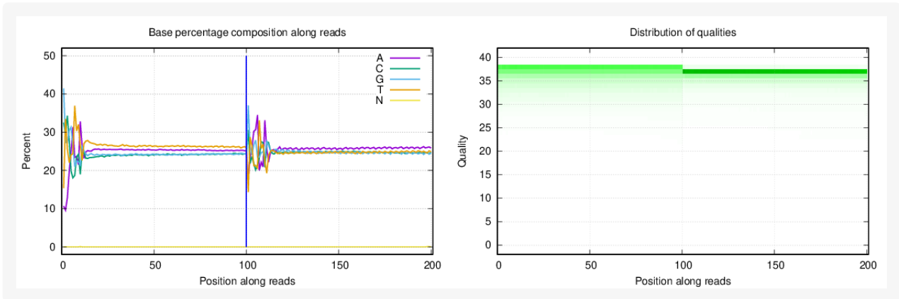
Figure 1-1 Distribution of base percentage and qualities of sample N12.
