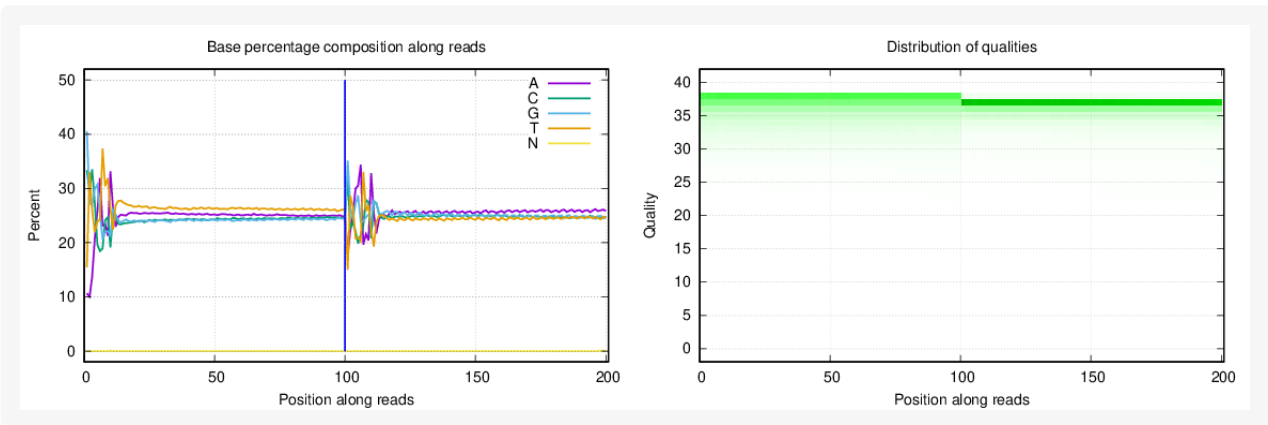
Figure 1-30 Distribution of base percentage and qualities of sample 7DR5.
