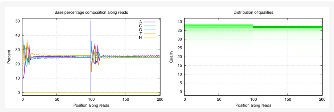
Figure 1-12 Distribution of base percentage and qualities of sample N1.
