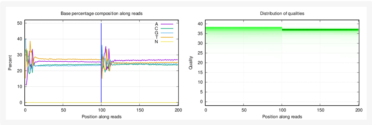
Figure 1-19 Distribution of base percentage and qualities of sample E6.
