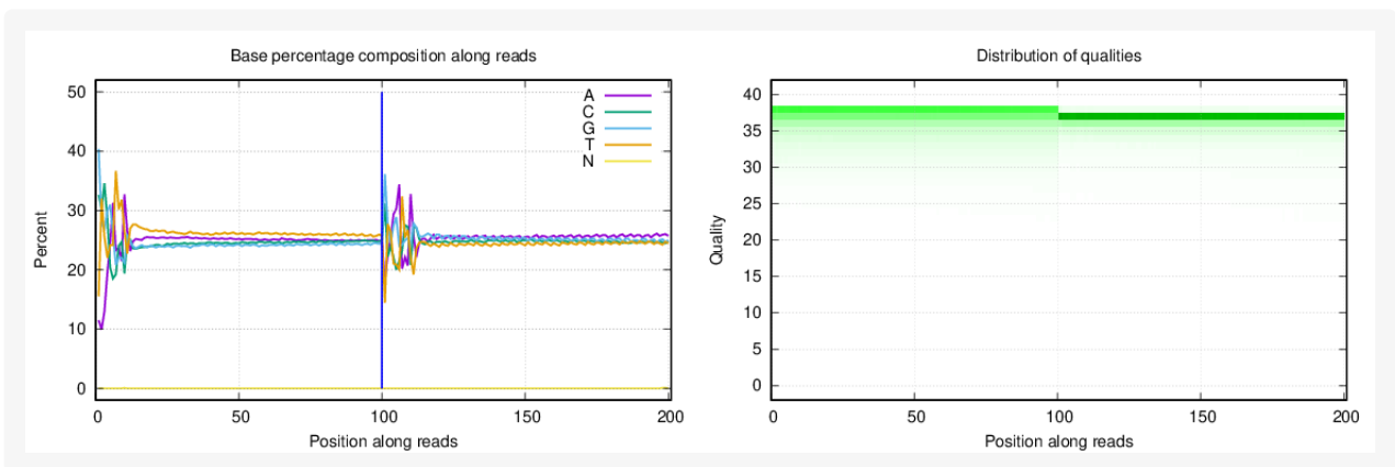
Figure 1-32 Distribution of base percentage and qualities of sample 15TR8.
