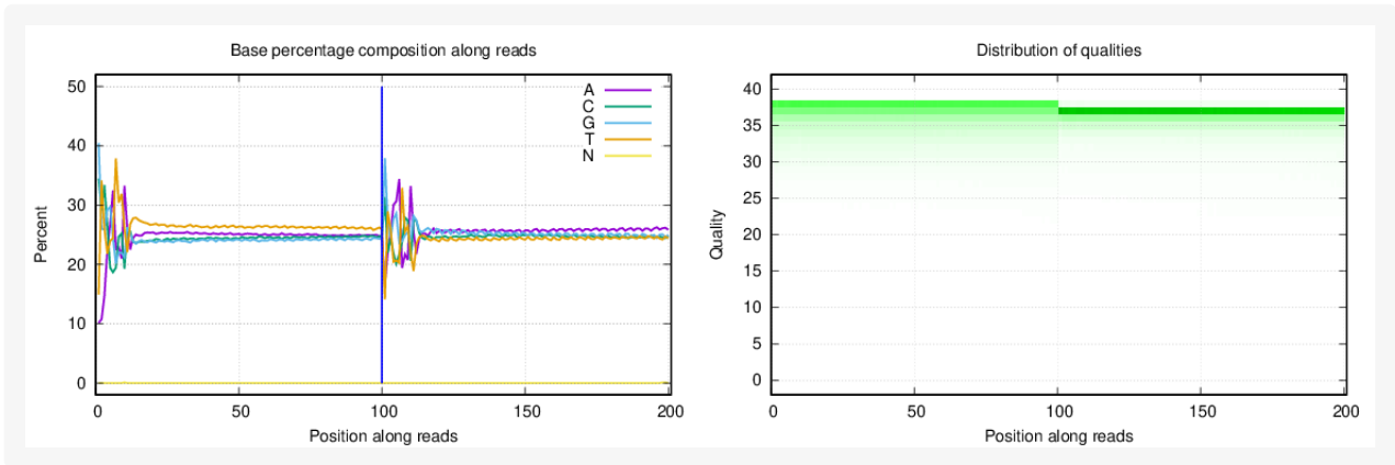
Figure 1-31 Distribution of base percentage and qualities of sample 15TR12.
