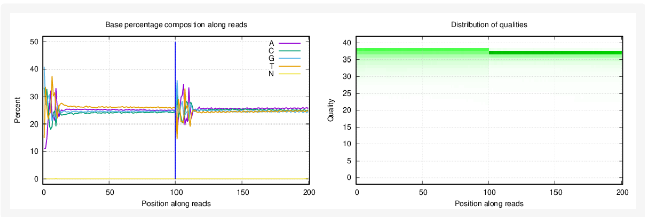
Figure 1-11 Distribution of base percentage and qualities of sample N2.
