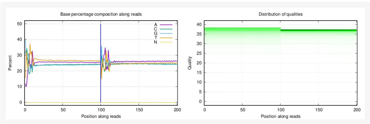
Figure 1-20 Distribution of base percentage and qualities of sample E5.
