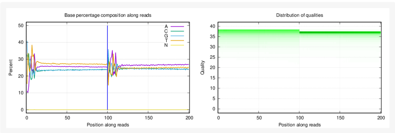
Figure 1-17 Distribution of base percentage and qualities of sample E8.
