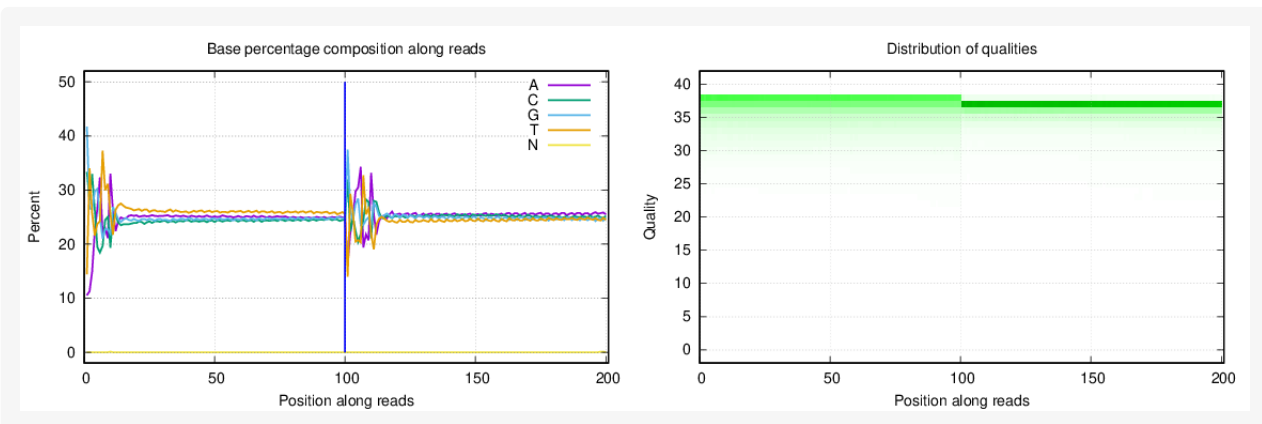
Figure 1-5 Distribution of base percentage and qualities of sample N8.
